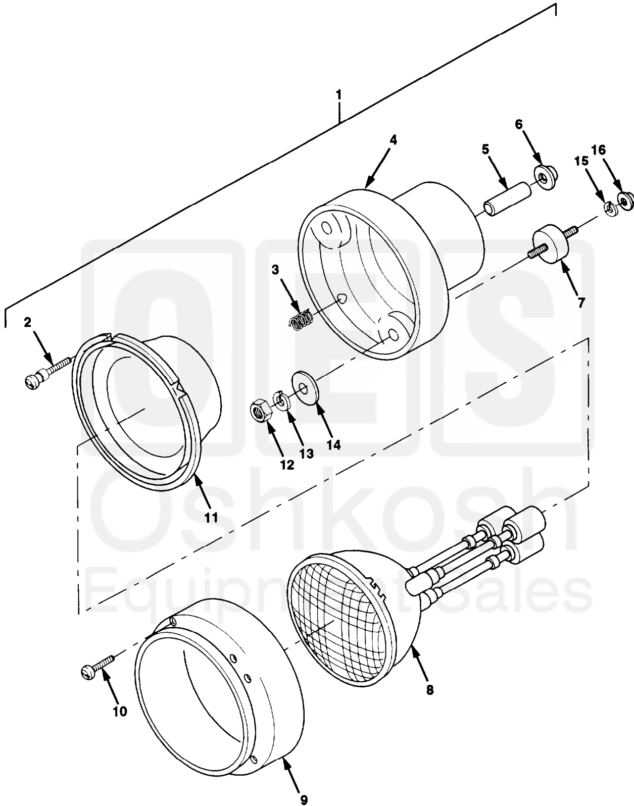
Figure 64. Headlight Assembly
